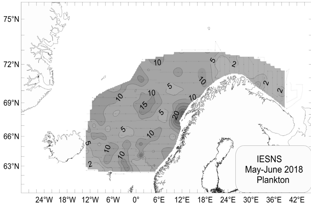
Figure 10. Representation of zooplankton biomass ( \text{g dry weight m}^{-2} ; at 0-200 m depth) in May-June 2018.
