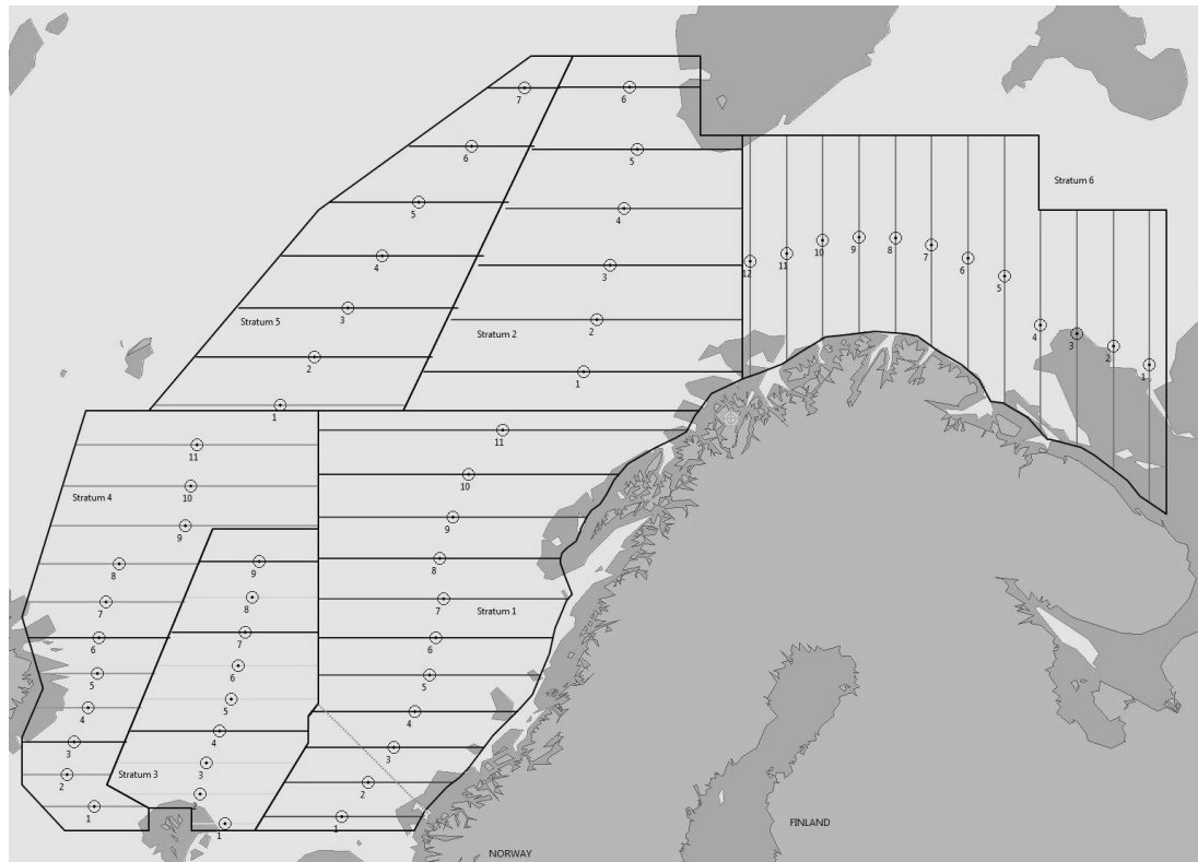
Figure 3. The pre-planned strata and transects for the IESNS survey in 2018 (red: EU, dark blue: Norway, yellow: Faroes Islands, violet: Russia, green: Iceland).
