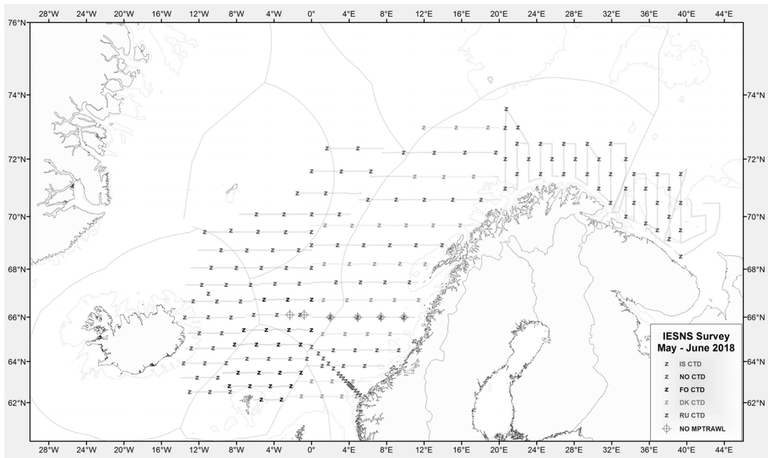
Figure 1. Cruise tracks and CTD stations by country for the IESNS survey in May-June 2018. Manta trawl hauls for sampling of micro plastics in the surface are also shown.
