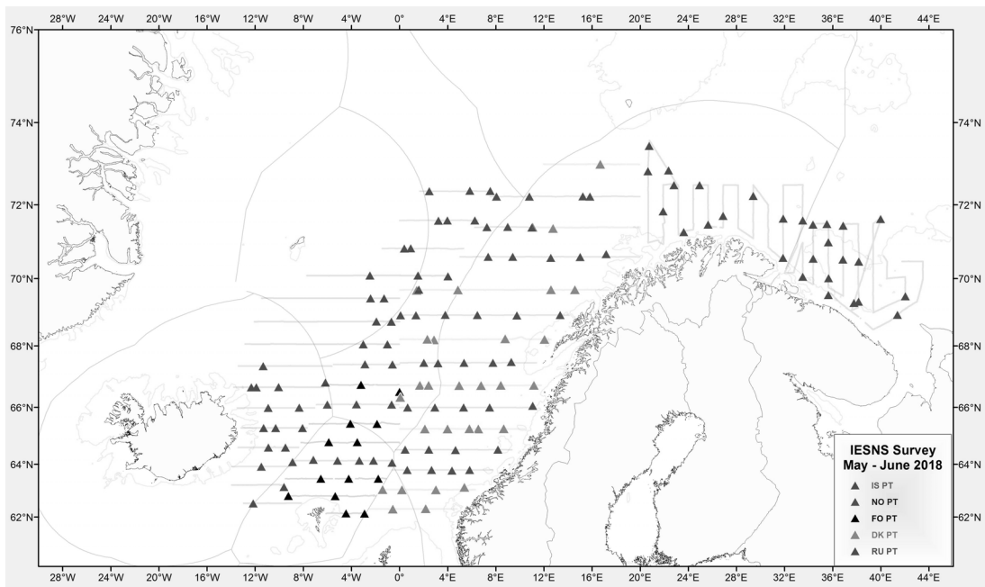
Figure 2. Cruise tracks during the IESNS survey in May-June 2018 and location of trawl stations.
